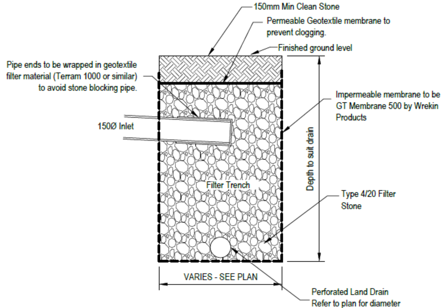
FILTER TRENCH CROSS SECTION
