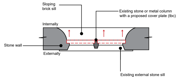
SCHEMATIC TYPICAL WINDOW PLAN
