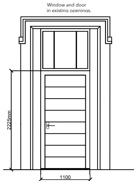
WINDOW TYPE 7 - (3 NO.) Above new rear doors on east elevation including fire escape on first floor.
