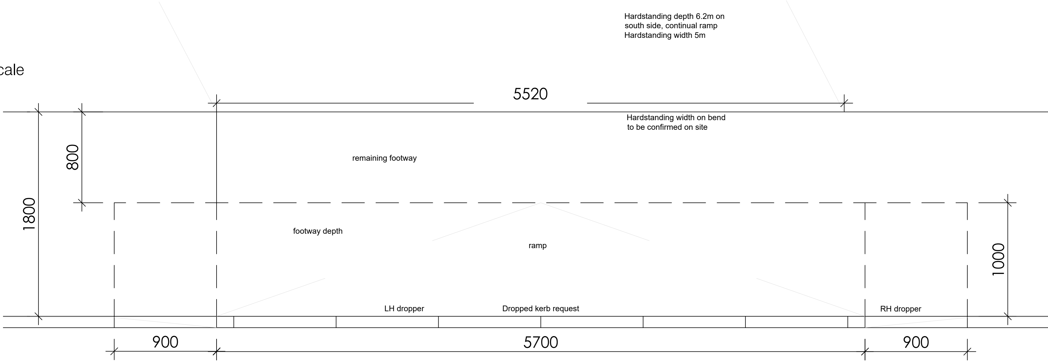
PROPOSED DROP KERB DIMENSIONS - 1:20 scale
