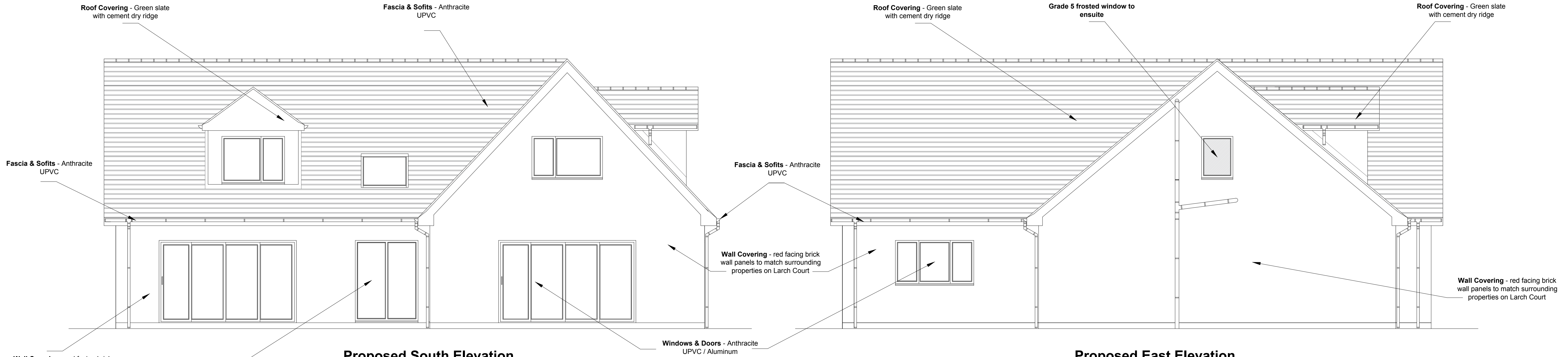
Proposed South Elevation
