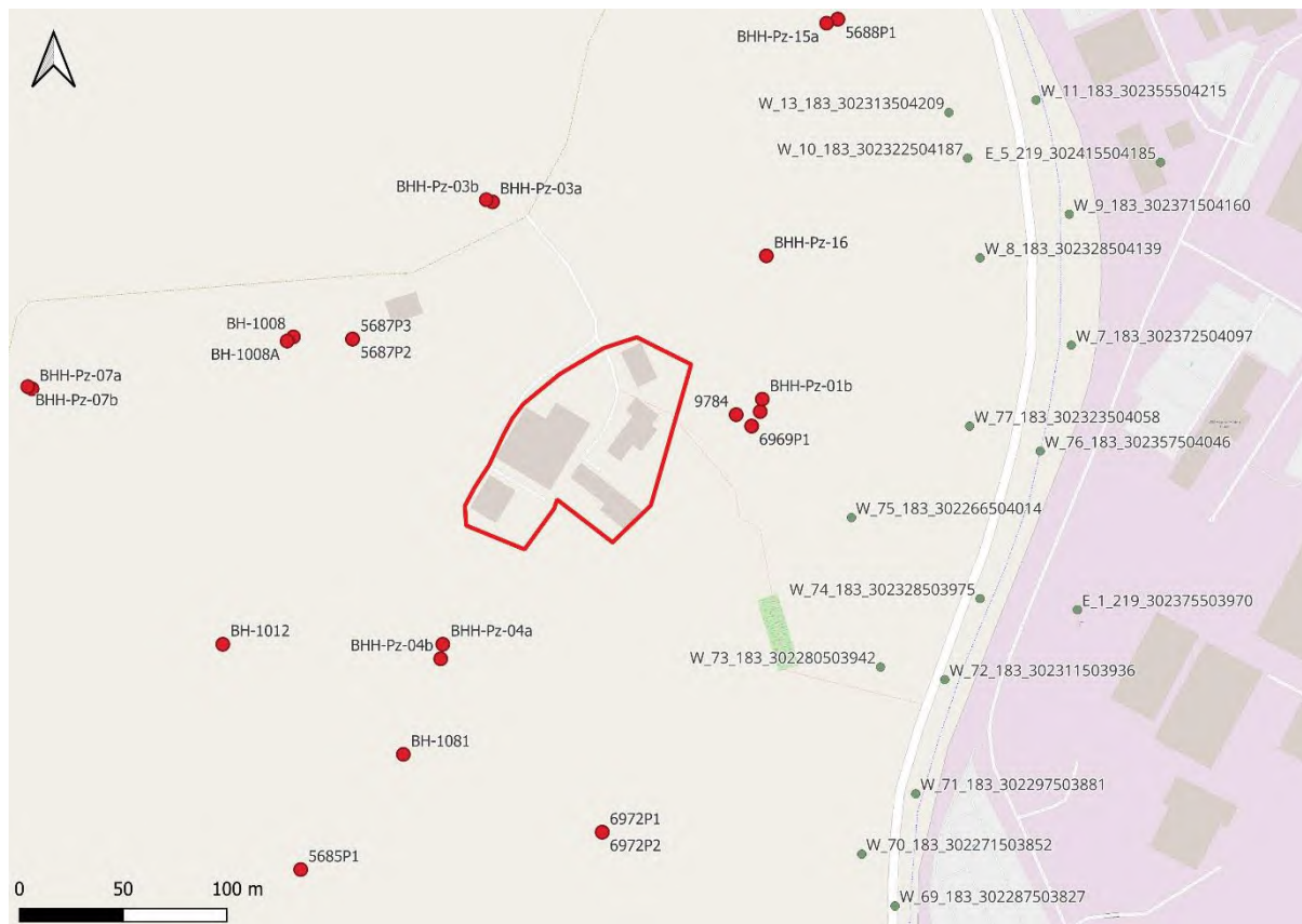
Figure 7 - Existing Borehole Records
