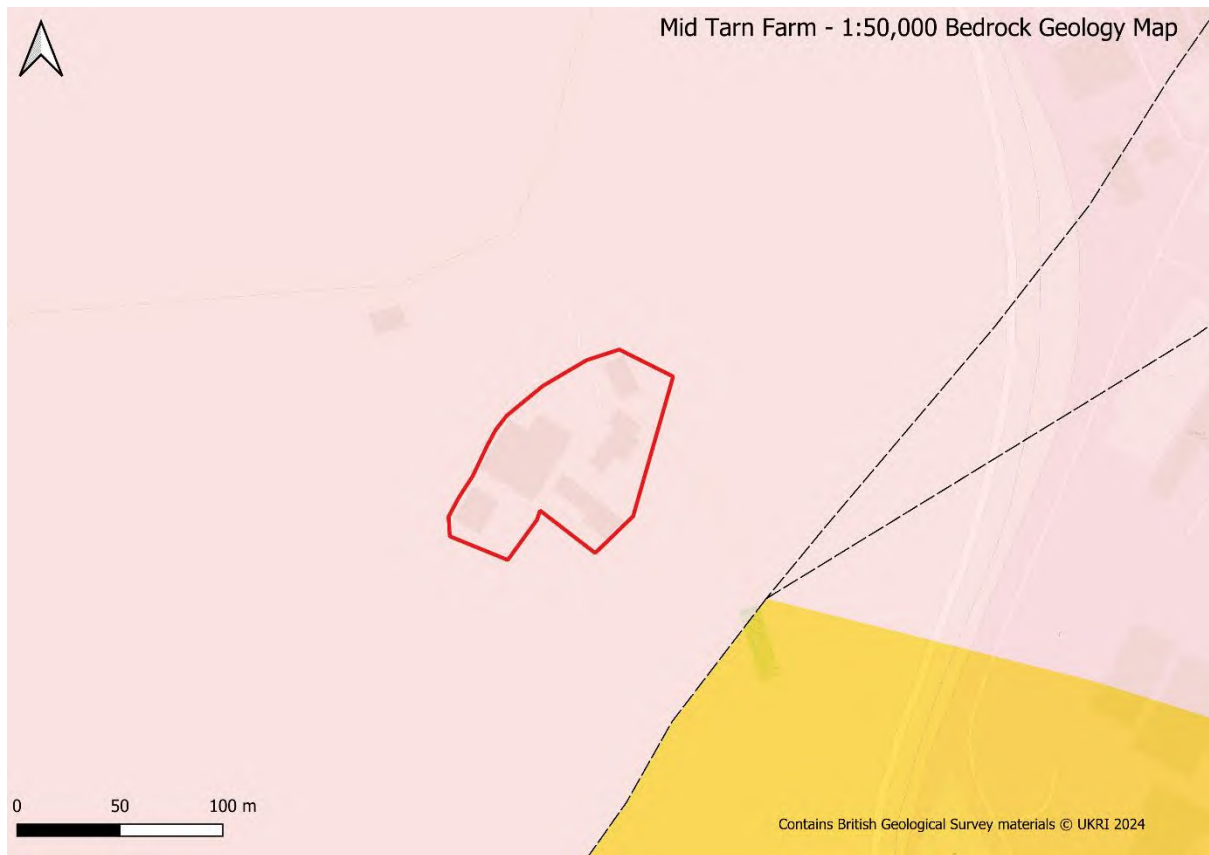
Figure 6 – BGS 1:50,000 Bedrock Geology Map and Linear Features (see table 4-2 for key)
