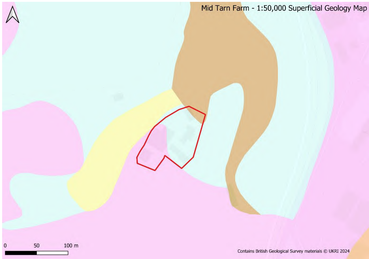
Figure 5 – BGS 1:50,000 Superficial Geology Map (see Table 4-1 for key)
