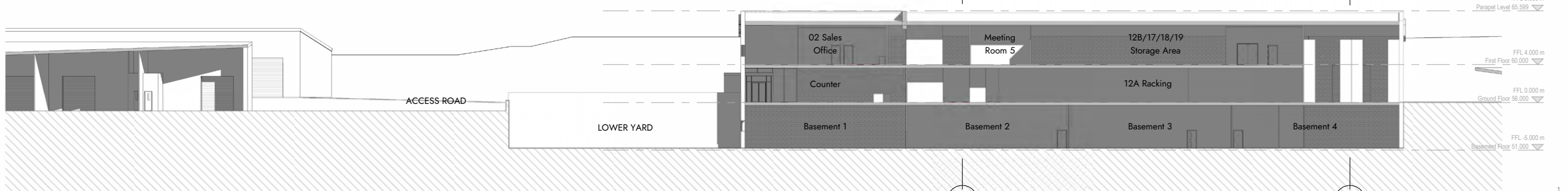
Site Section DD - Thro' Units 4 to 6 and Main Building 1 : 200
