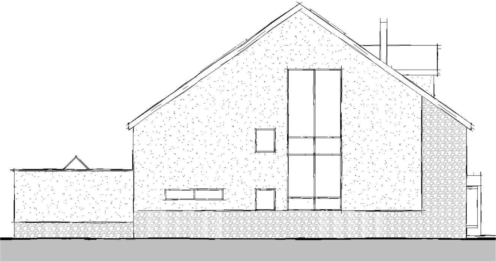
Side Elevation 02 1 : 100
