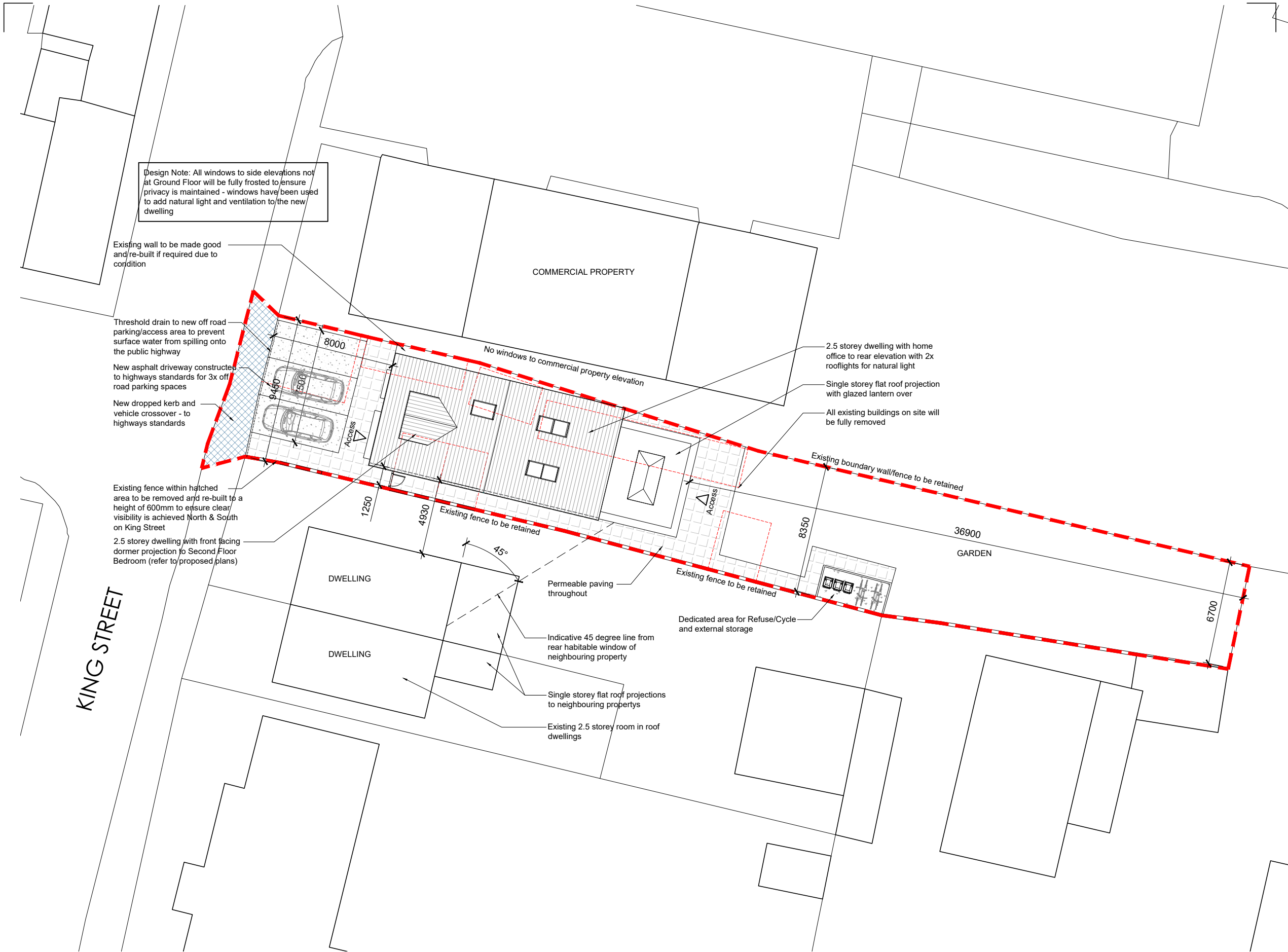
△ PROPOSED SITE PLAN @ 1:250
