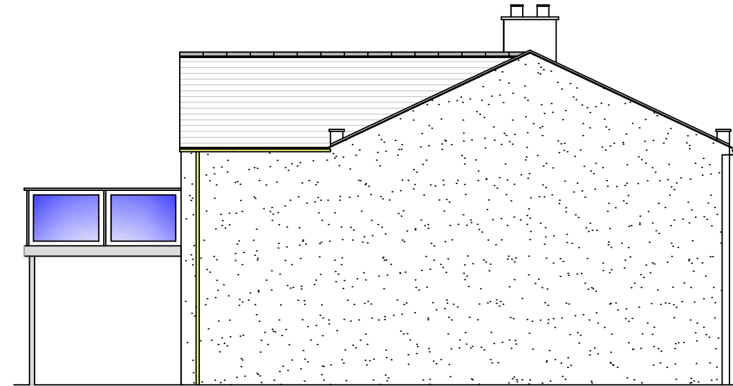
East Elevation
