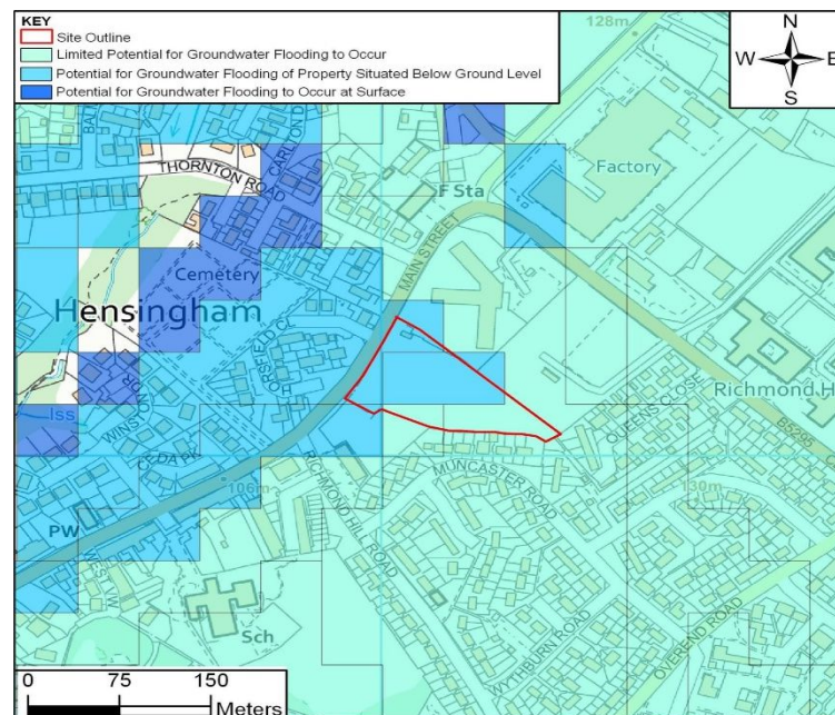
Figure 3.6.1 British Geological Society Ground Water Flood Map
