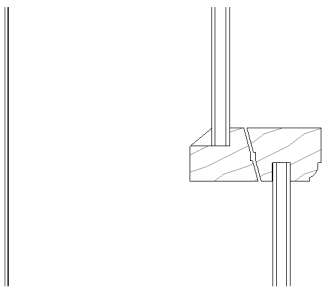
Sash Detail ZZ-DR-A-31309 SCALE: 1 : 5
