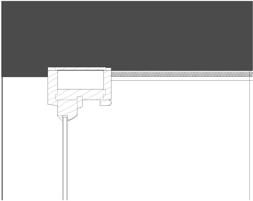
Head Detail ZZ-DR-A-31309 SCALE: 1 : 5
