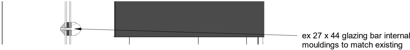
Moulding Detail ZZ-DR-A-31309 SCALE: 1 : 5
