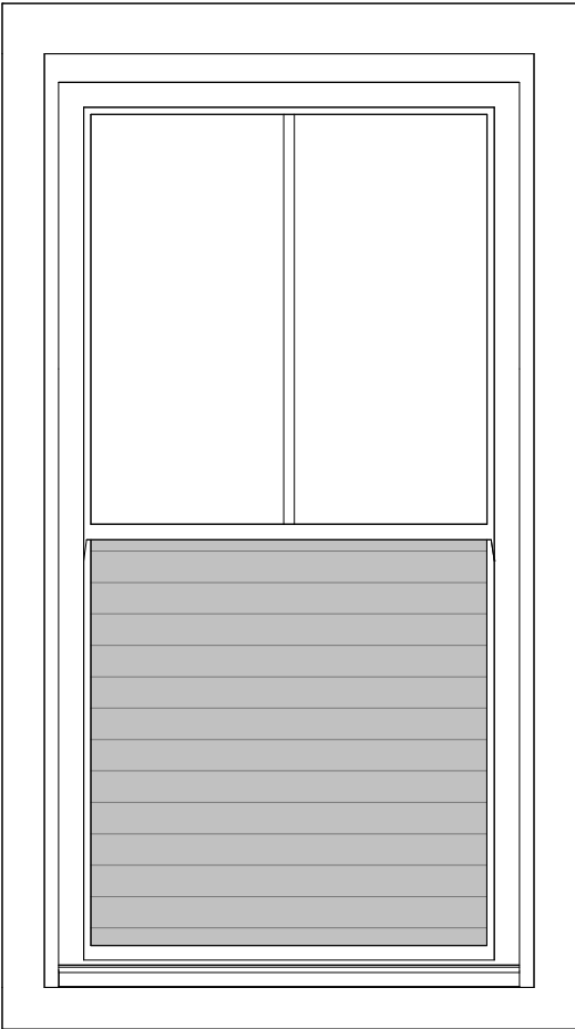
Elevation External ZZ-DR-A-31308 SCALE: 1 : 20
