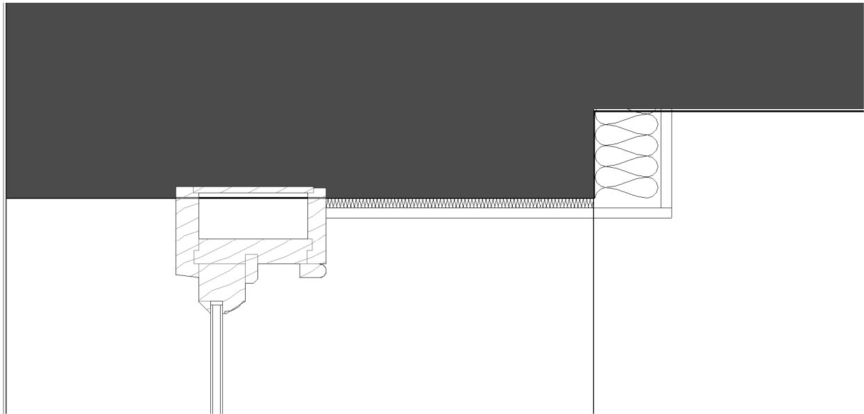
Head detail ZZ-DR-A-31308 SCALE: 1 : 5
