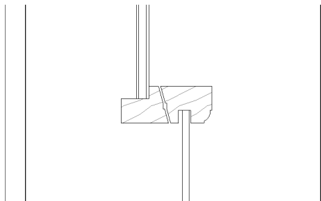
Sash detail ZZ-DR-A-31307 SCALE: 1 : 5
