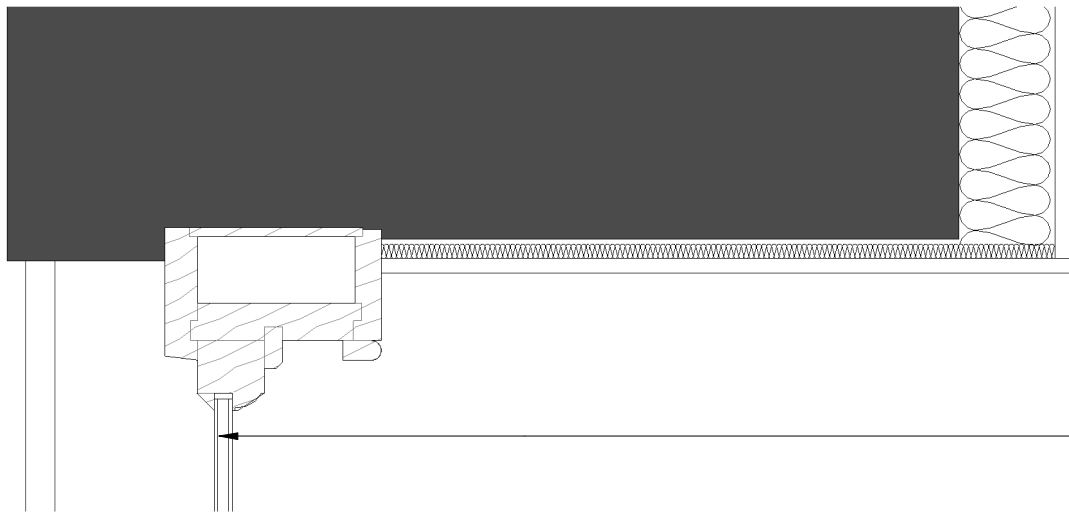
Head detail ZZ-DR-A-31307 SCALE: 1 : 5
