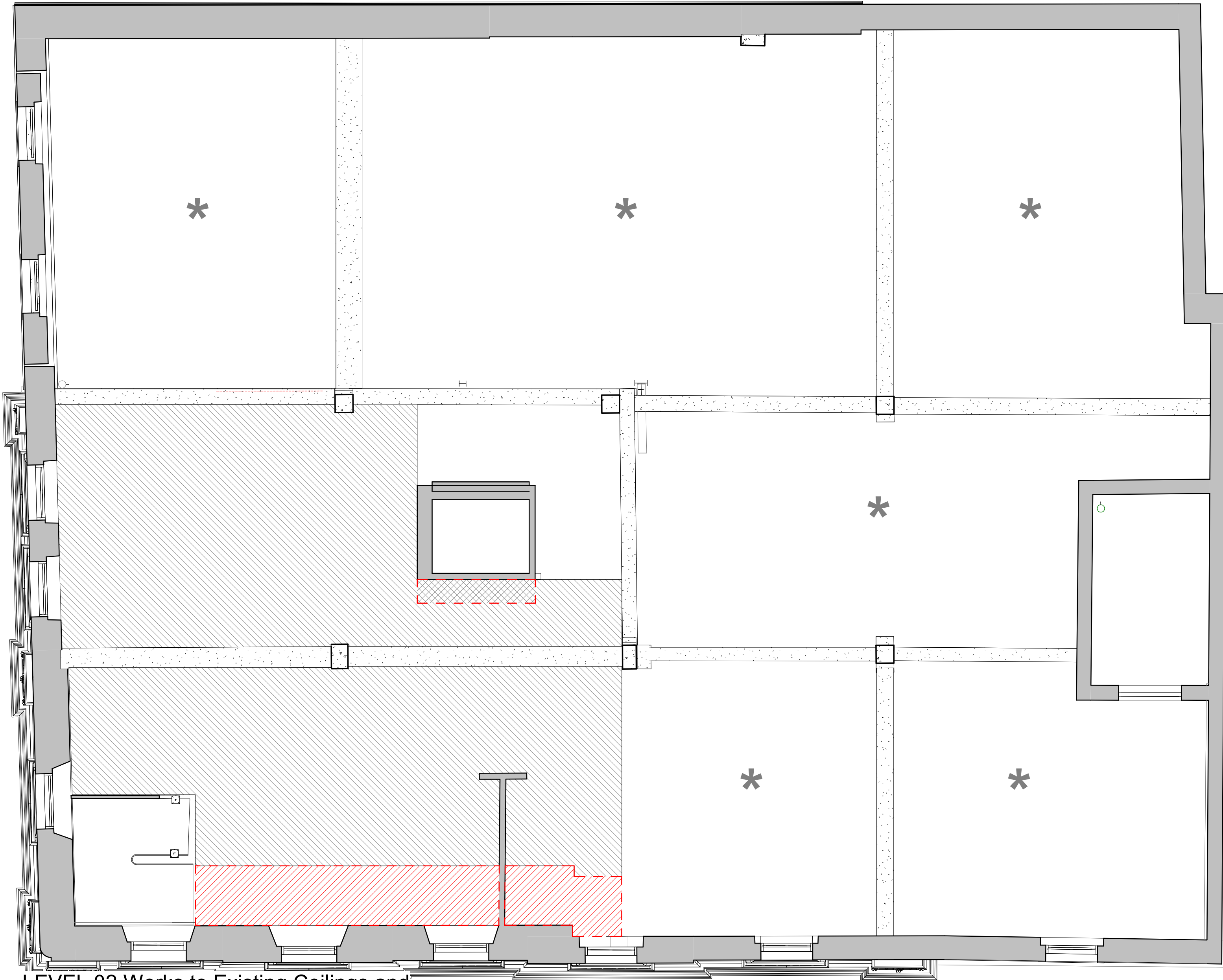
LEVEL 02 Works to Existing Ceilings and walls N.T.S.
