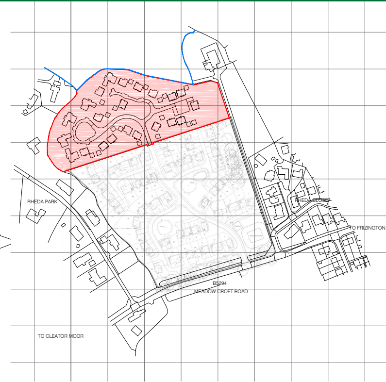
location plan 1:1250 @ A1 / 1:2500 @ A3 SITE AREA: 20902m2 / 5.164 Acres.
