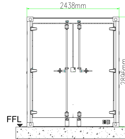
Concrete Base Right View
