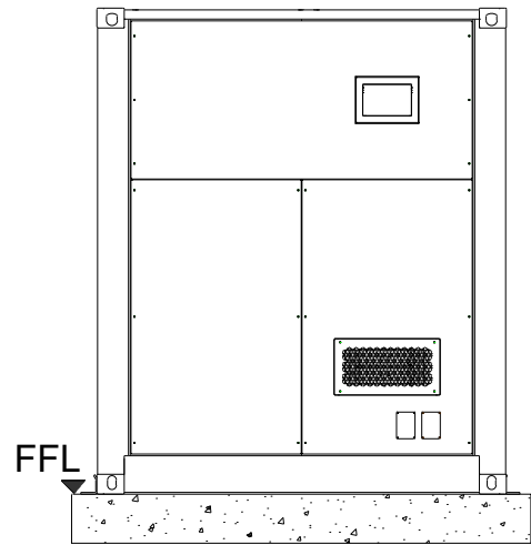
Left view
