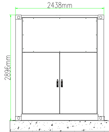
Right view
