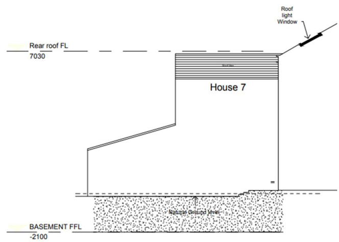
Elevation 7a (house 7 side elevation)
