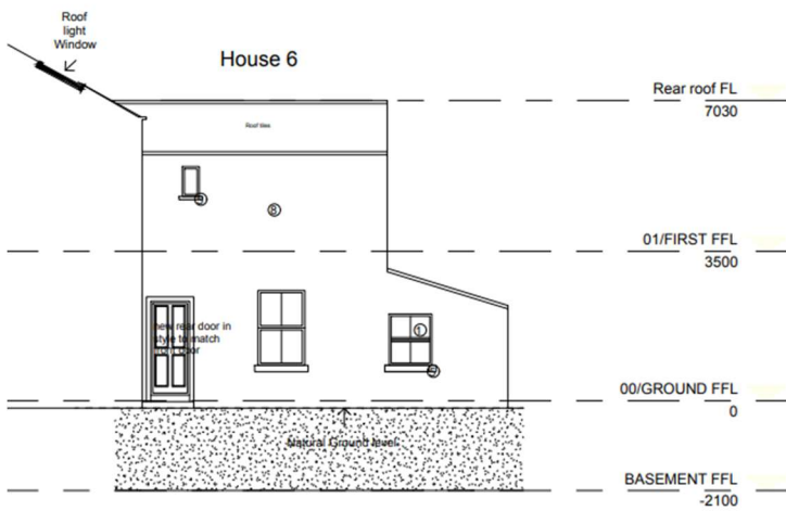
Elevation 6 (house 6 side elevation) 1 : 100
