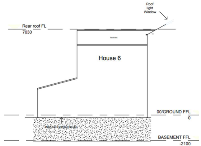
Elevation 6a (house 6 side elevation) 1 : 100
