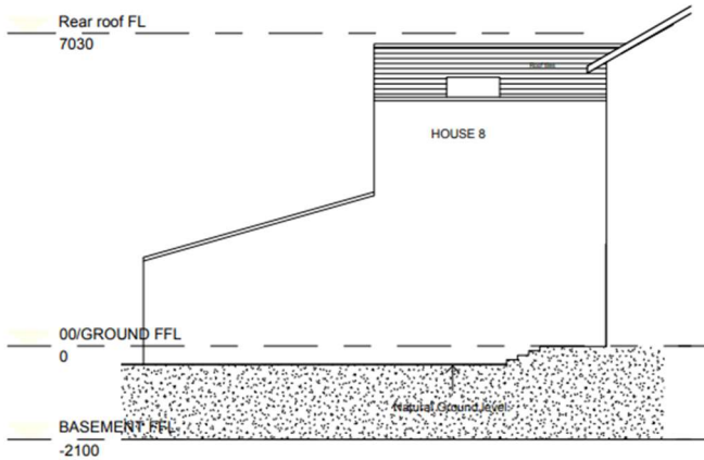
Elevation 8a (house 8 side elevation) 4 - 100
