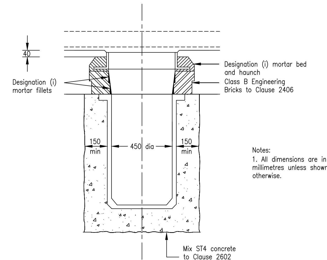
DETAIL 1 – TRAPPED STREET GULLY
