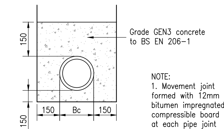
Class Z Bedding PIPE WITH COVER LESS THAN 1.2m & GULLY CONNECTIONS
