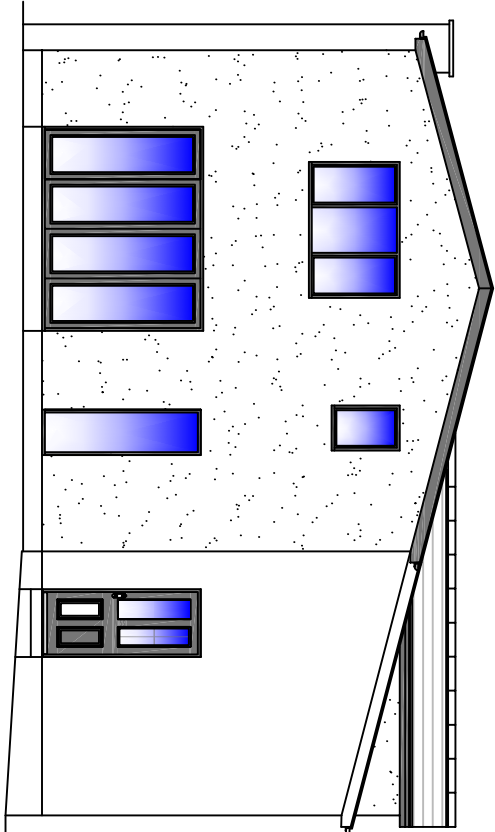
North Elevation
