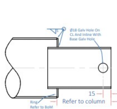
Spigot Detail
