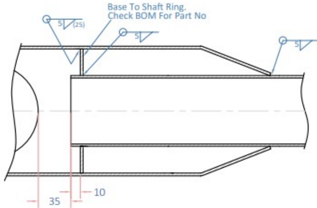
Swage Detail
