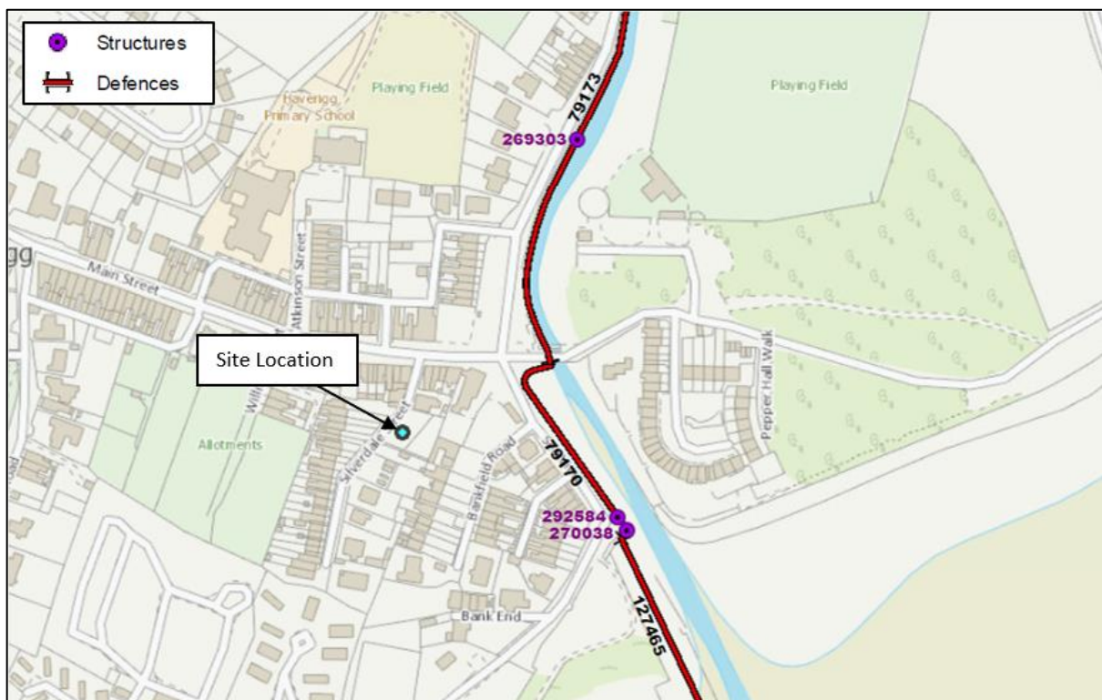
Figure 9 Map of existing flood defences and location of site (Source: EA)
