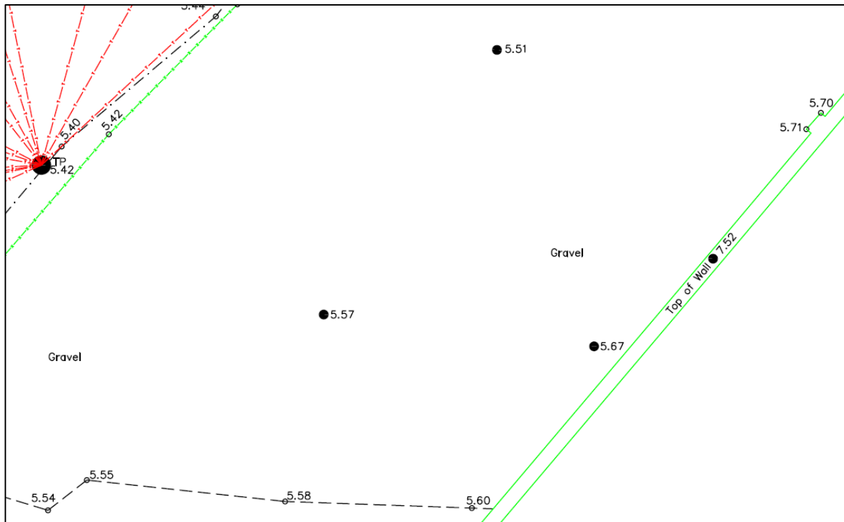
Figure 13: Extract from topographic survey, providing evidence of approximate topographic levels within southern part of site
