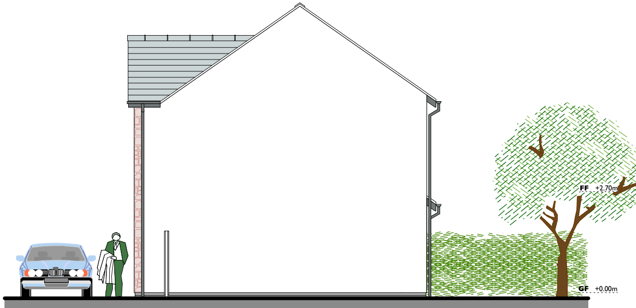
Side Elevation 1:100
