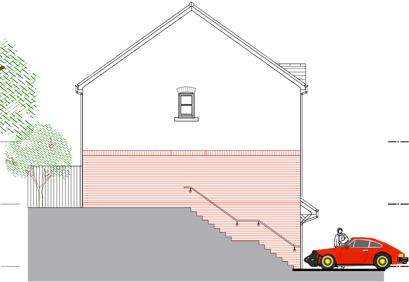
Side Elevation
