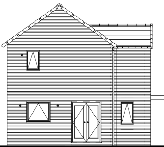
REAR ELEVATION
