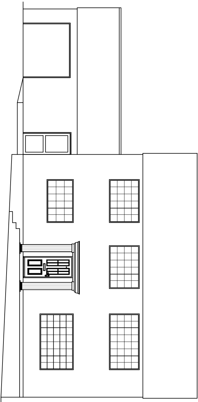
West Elevation
