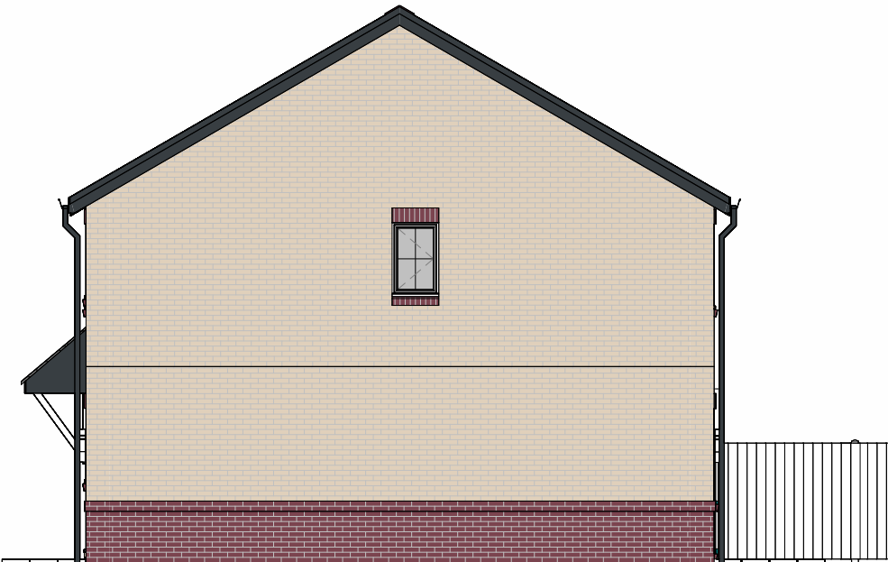
Side Elevation 1:100
