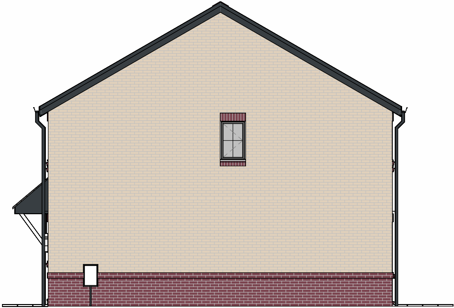
Side Elevation 1:100
