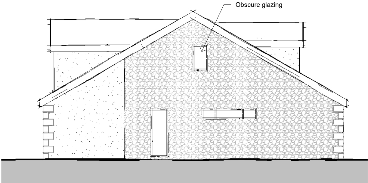
Side Elevation 02 1 : 100
