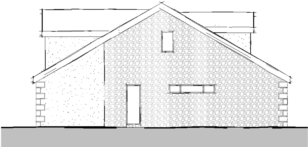
Side Elevation 02 1 : 100
