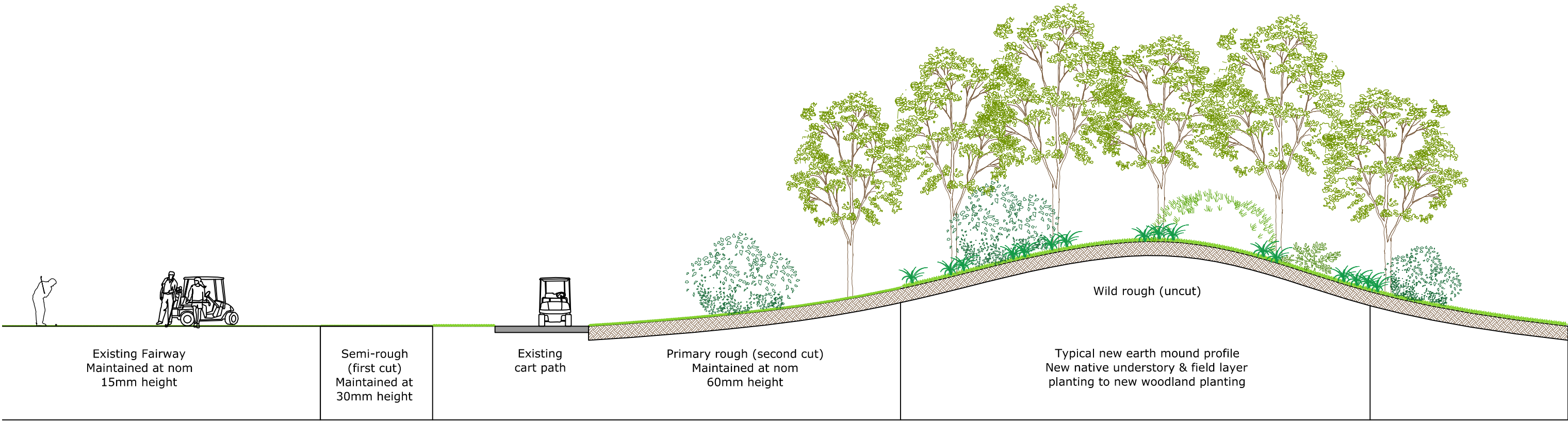
TYPICAL SECTION - Scale 1:125
