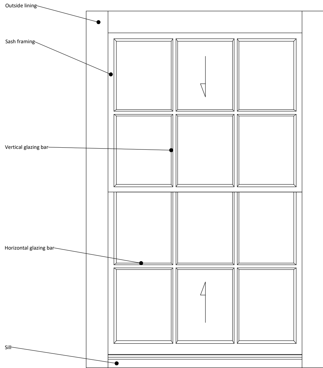
Window External Elevation
