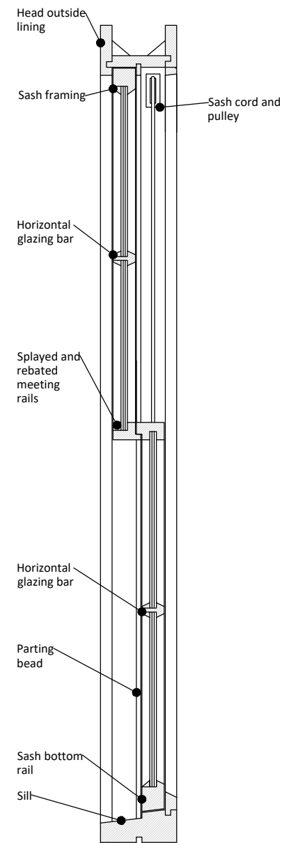
Vertical Section Through Window
