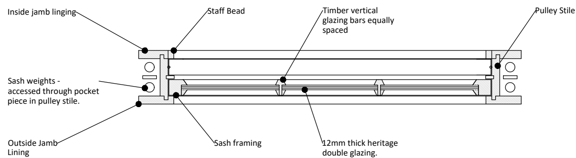
Horizontal Section Through Window
